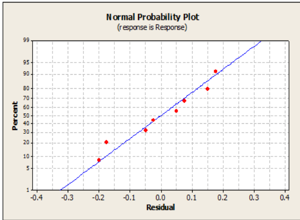
Figure 3: Normal Probability Plot
