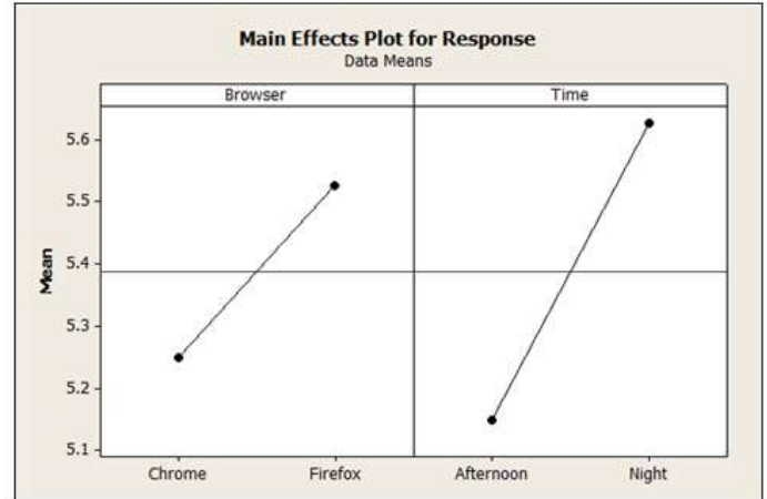
Figure 5: Main Effects after Blocking
