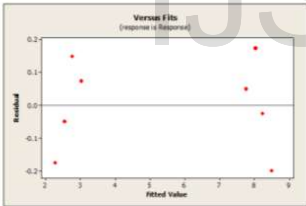
Figure 4: Residual vs Fits
